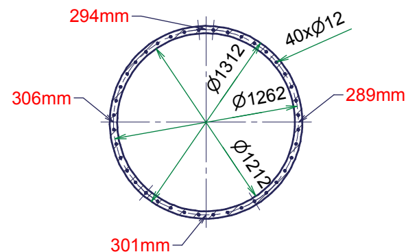
U-U ( 1 : 25 ) OUTLET FLANGE
